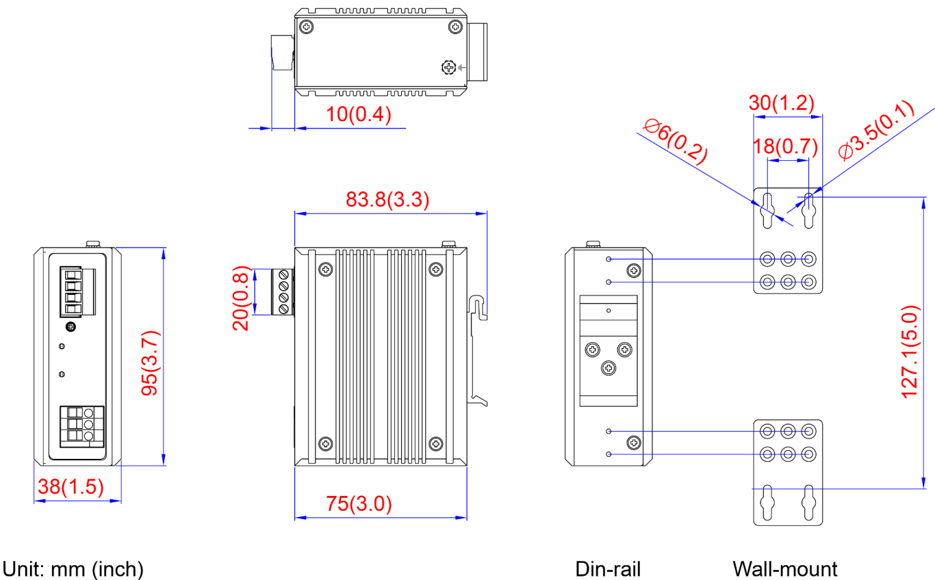
Figure 2.1 - Physical Dimensions
