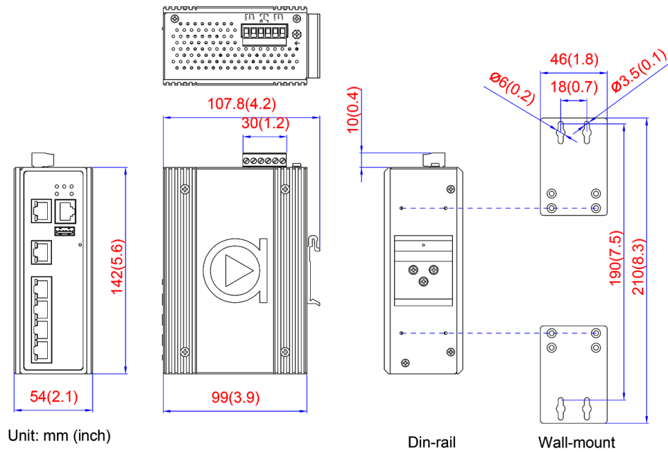
Figure 2.1 - Physical Dimensions
