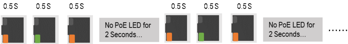
Figure 2.8 - PoE Cable Short LED Sequence
