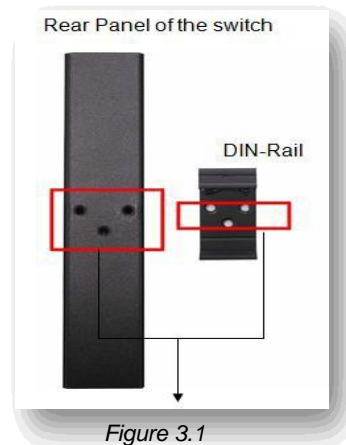
The Rear Side of the Switch and DIN-
