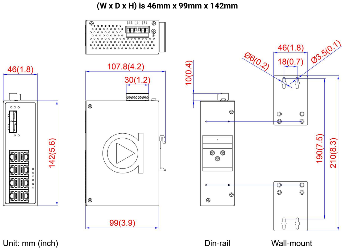
Figure 2.1 - Physical Dimensions
