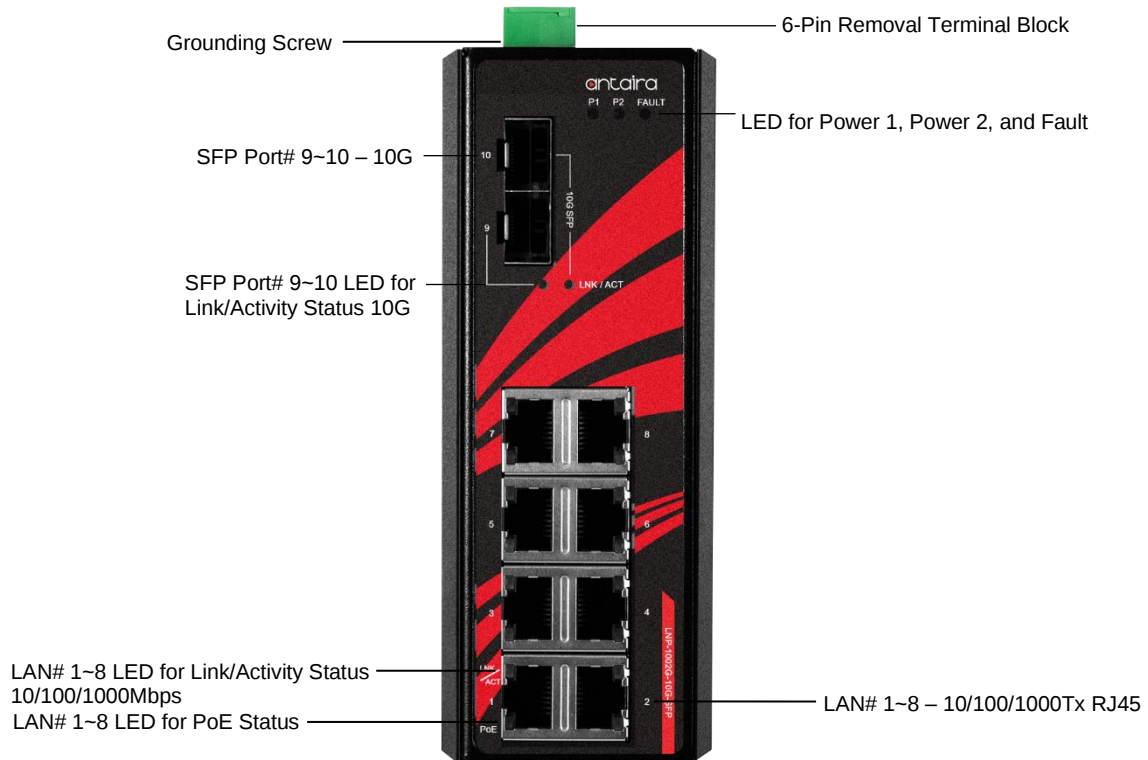
Figure 2.2 - The Front Panel of LNP-1002G-10G-SFP
