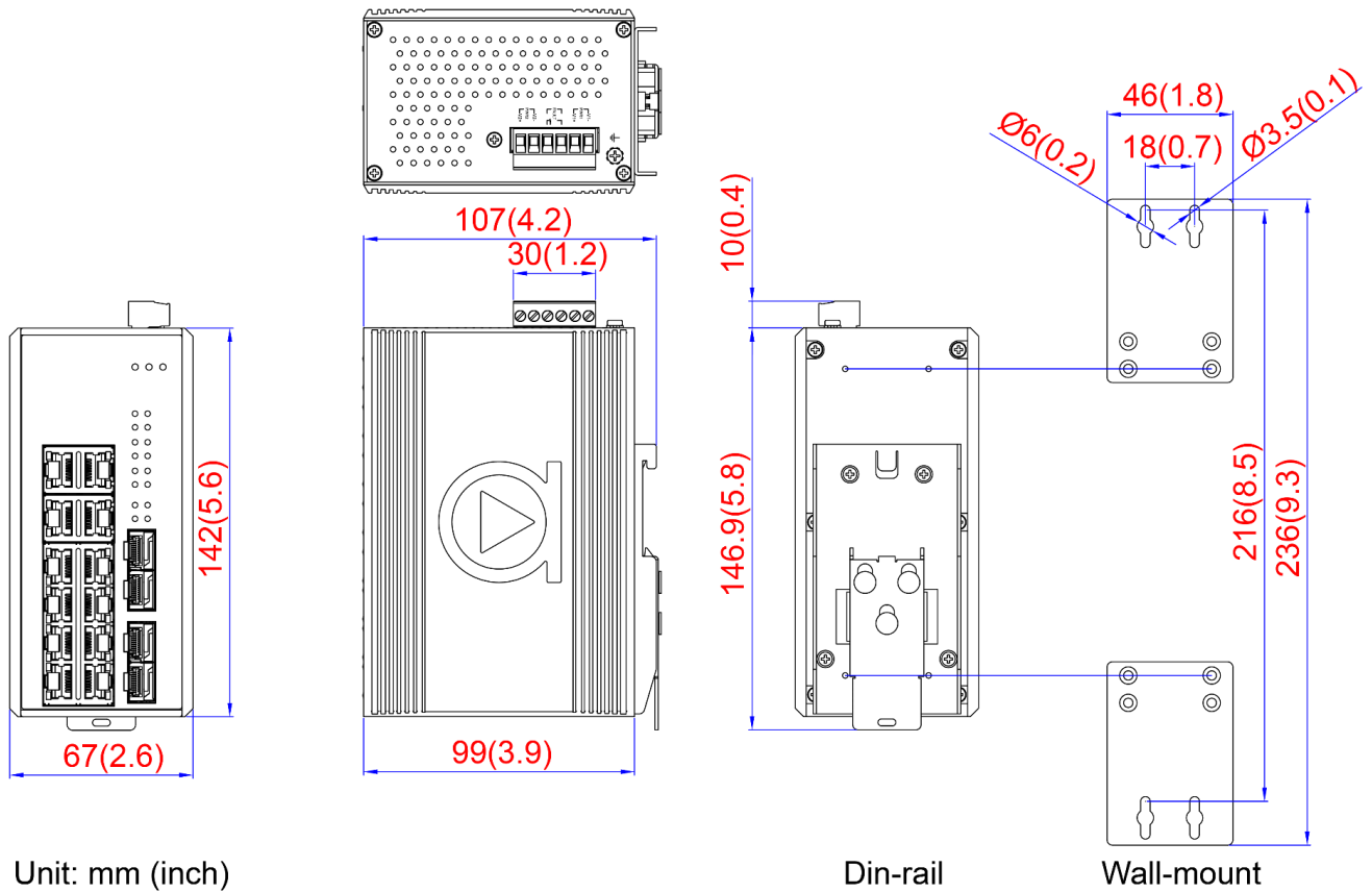
Figure 2.1 - Physical Dimensions
