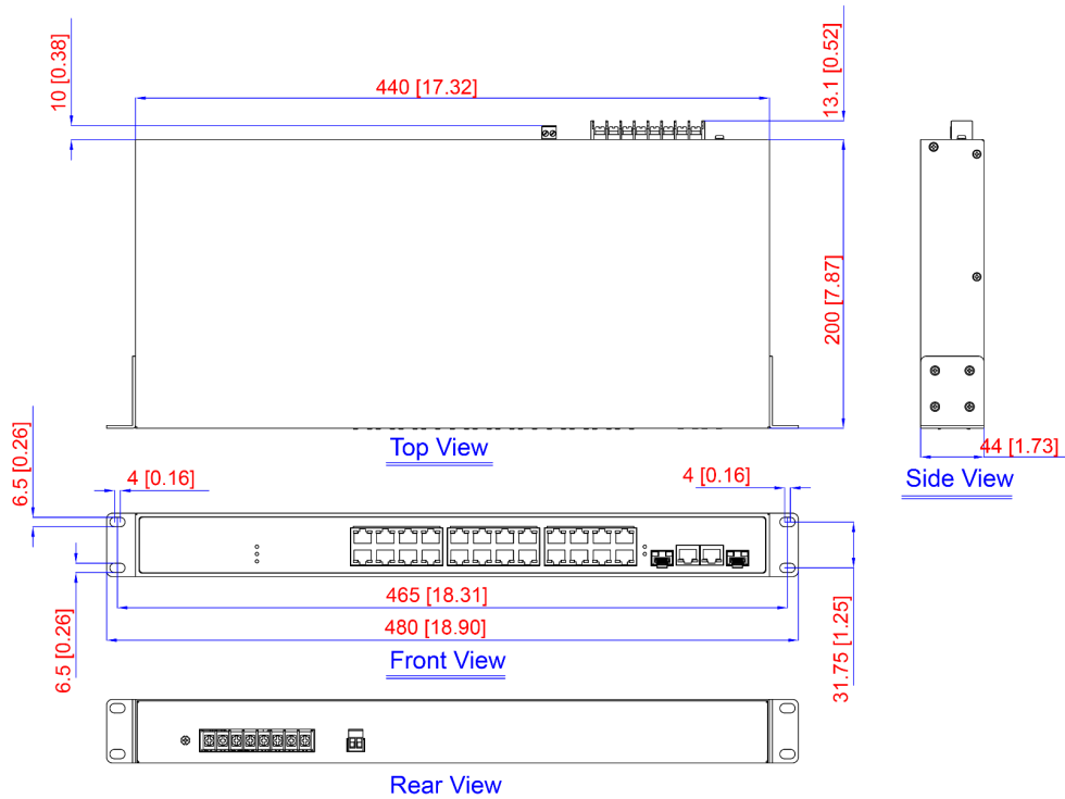
Figure 2.1 - Physical Dimensions
