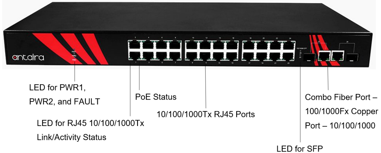
Figure 2.2 - Front View Panel
