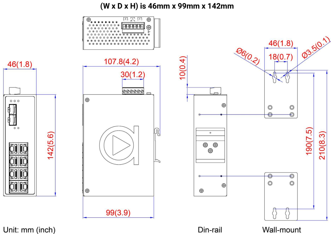
Figure 2.1 - Physical Dimensions
