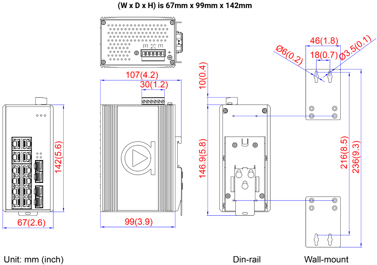
Figure 2.1 - Physical Dimensions
