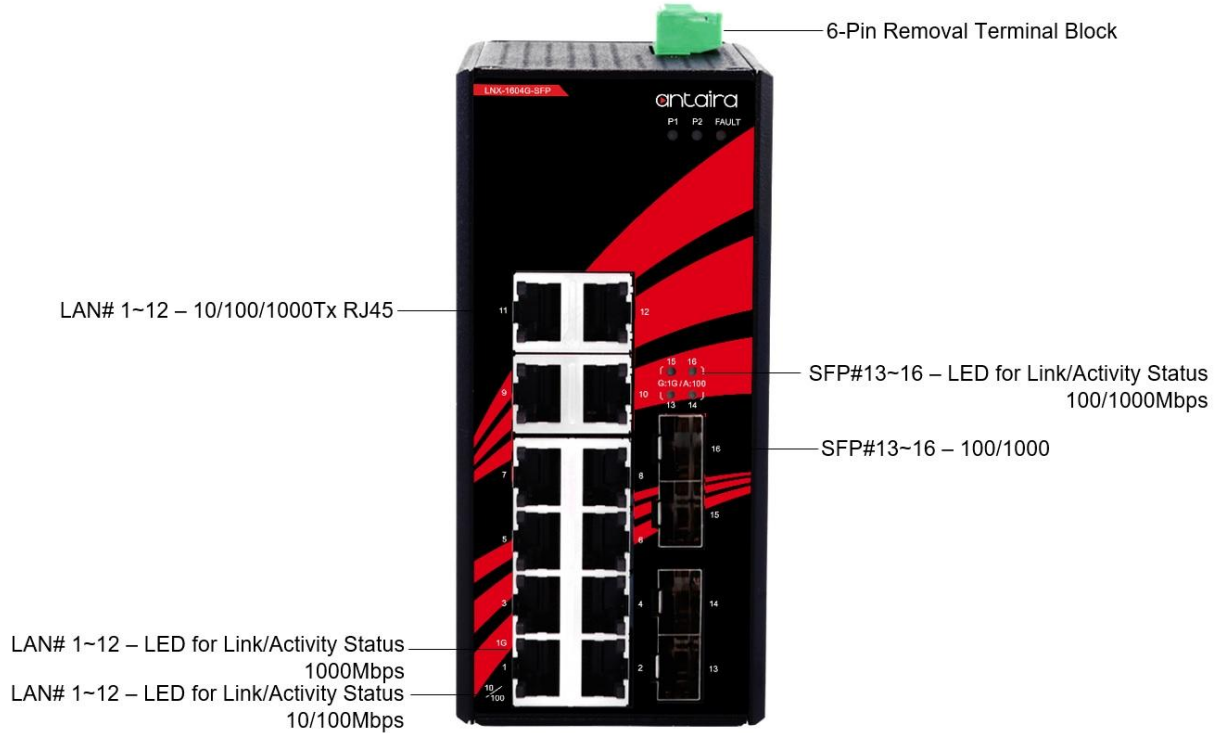
Figure 2.2 - Front View Panel
