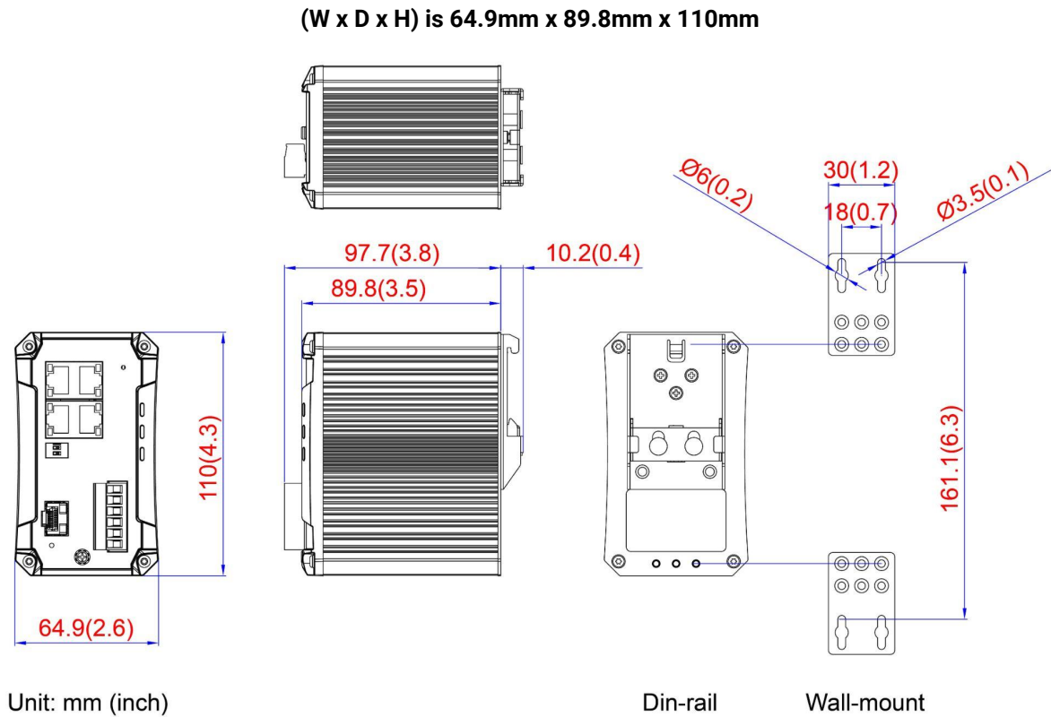
Figure 2.1 - Physical Dimensions
