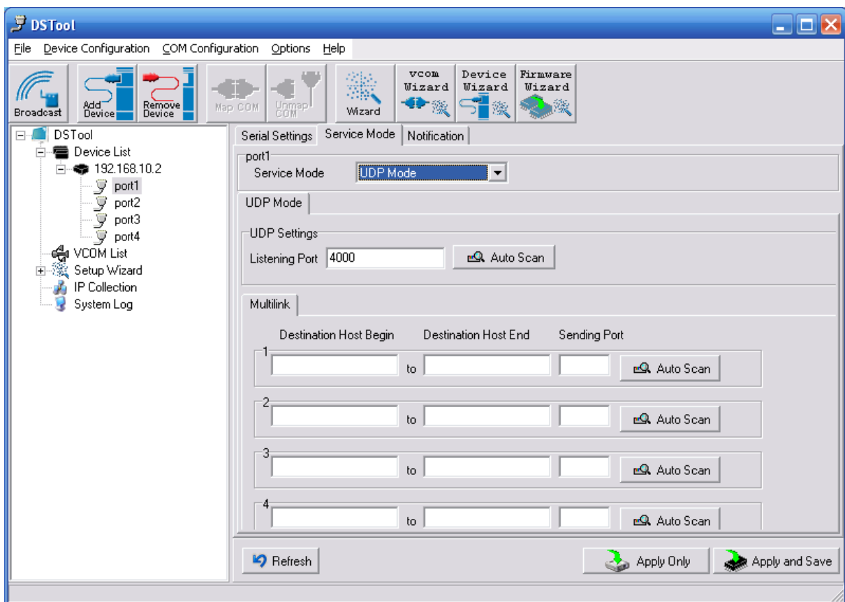
Figure 5-15 UDP mode
