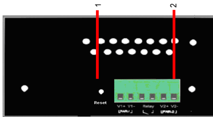
Figure 3-2 Bottom Panel
