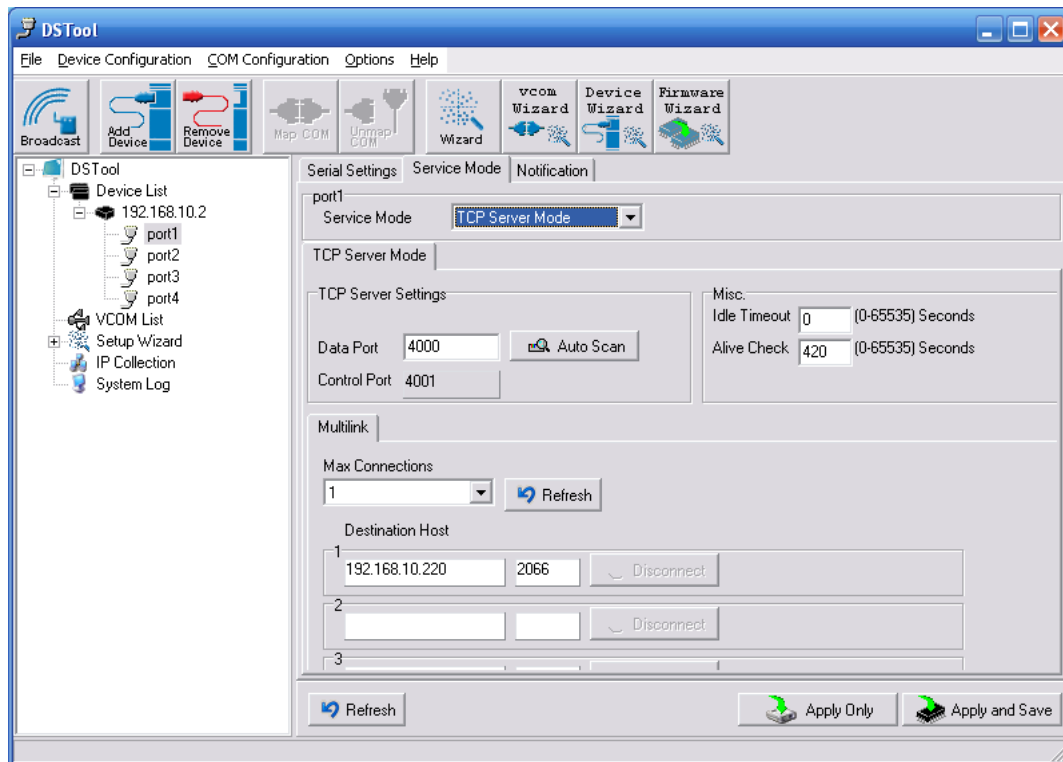
Figure 5-13 TCP Server mode
